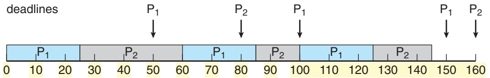
Figure 6.19 Earliest-deadline-first scheduling.
